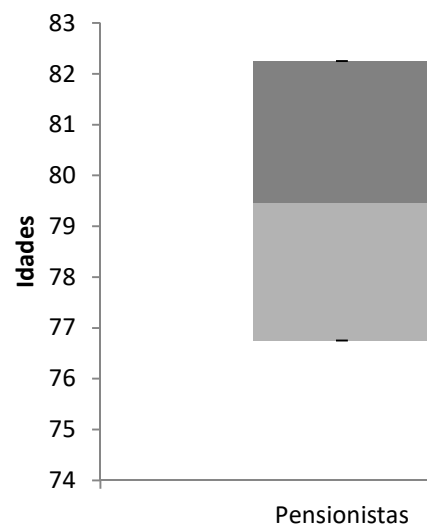
BOXPLOT PENSIONISTAS
